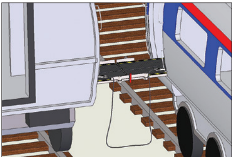
Figure 1-8 – Unfold transfer bridge to flat position and insert Safety Lock Bar with red handle up.
